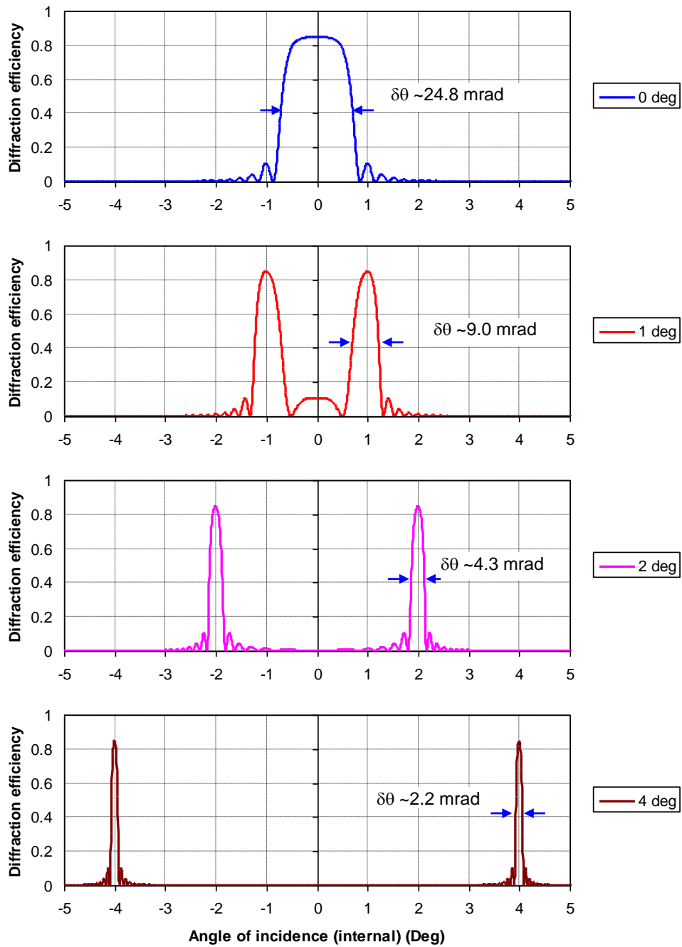
Fig. 4. Calculated diffraction efficiency vs. internal angle of incidence for VBG elements at the same resonance wavelength (2051 nm) and the same reflectivity maximum (R~85%) but different Bragg angle (0, or 1, or 2, or 4 deg). 0 deg corresponds to normal incidence. Both “+” and “-” diffraction orders are shown for angles of incidence other than 0 deg. At normal incidence both orders merge into one peak providing the largest angular acceptance.
