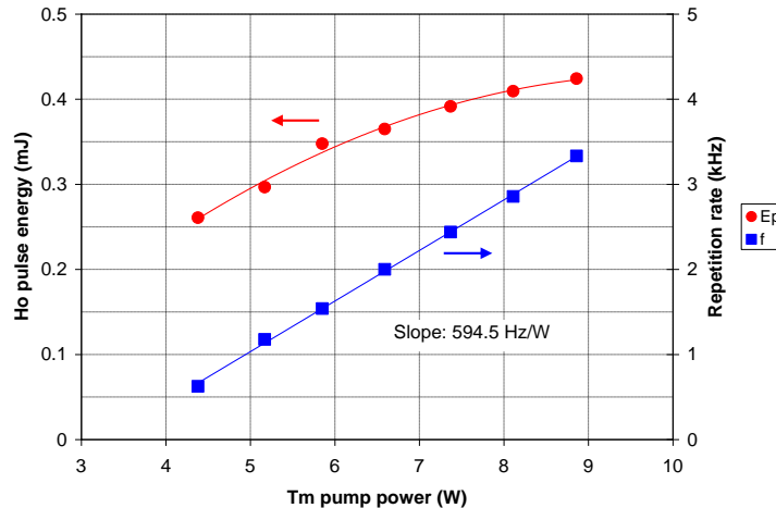
Fig. 6. Pulse energy (circles) and repetition rate (squares) vs. pump power for a ring Ho:YLF oscillator with VBG output coupler and ~95%-transmissive Cr 2+ :ZnSe saturable absorber.
