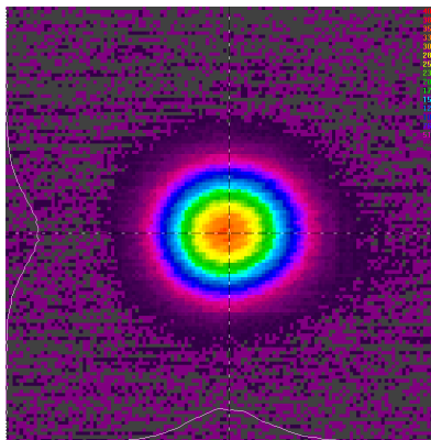
Fig. 5. Measured profile for the free-propagating beam from the Ho:YLF ring laser at maximum pump power. The beam full width and fit to Gaussian are 4.5 mm and 0.95 for horizontal direction and 4.0 mm and 0.96 for vertical direction, respectively.
