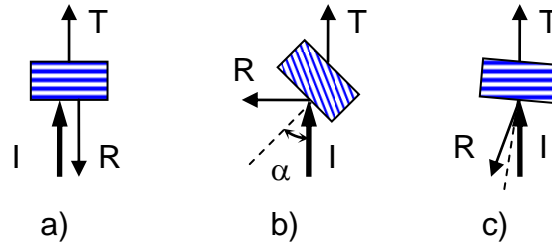
Fig. 1. Operation of thick holographic gratings in laser resonators: a) Normal incidence – provides maximum angular acceptance and is utilized in standing-wave resonators, b) Large angle of incidence in the range of 5 to 85 deg – more than 10x reduction in angular acceptance vs. normal incidence, c) Small angle of incidence 0.5-2 deg – only 2-5 times reduction in angular acceptance vs. normal incidence (this work).
