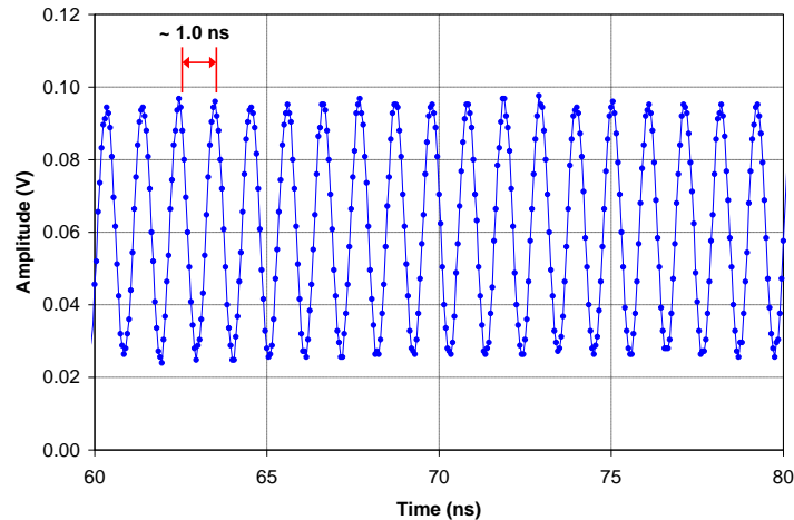
Fig. 8. High-resolution view (20-ns-wide window) of a multi-frequency laser pulse trace in Fig. 7b. The data point interval is 50 ps.
