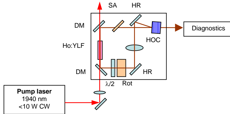
Fig. 2. Schematic layout of the ring Ho:YLF oscillator (HOC –holographic output coupler, SA – saturable absorber, DM – dichroic mirror, HR – high reflector, Rot - Faraday rotator).
