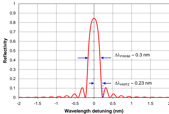
Fig. 3. Calculated reflectivity at normal incidence vs wavelength detuning for a VBG element with resonance wavelength of 2051 nm, ~7-mm thickness and 150-ppm index modulation. The full-width at half-maximum (FWHM) for the reflectivity peak is ~0.3 nm. The half-width at first zero (HWFZ) is ~0.23 nm.
