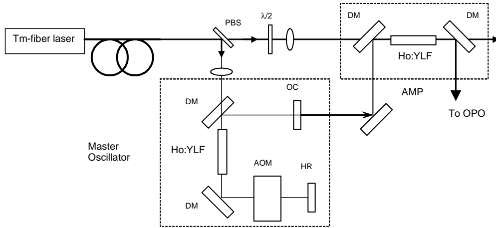
Fig. 1. Schematic layout of the end-pumped Ho:YLF MOPA (PBS – polarizing beam splitter, DM – Dichroic Mirror, AOM – Acousto-Optic Modulator, OC – Output Coupler, HR – High Reflector).
